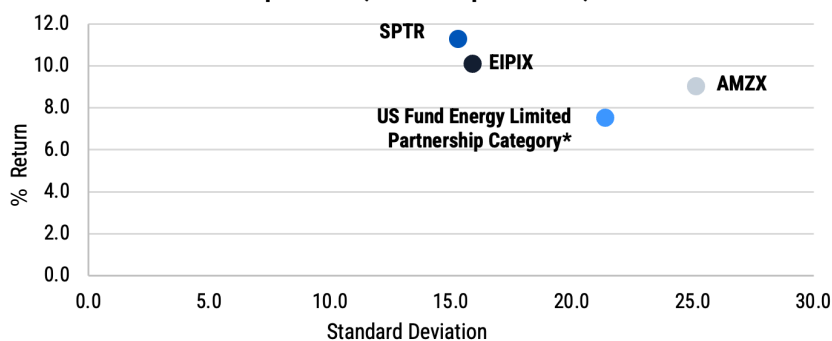
Risk Return Scatter Plot September 1, 2006 - September 30, 2026
